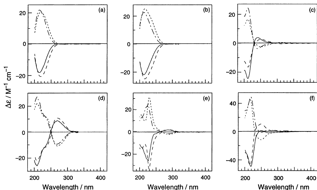
Fig. 5. CD spectra of (–)– and (+)–quadracyclanes in hexane (solid and chain, respectively) and in acetonitrile (dash and short dash, respectively): (a) 1b , (b) 2b , (c) 3b , (d) 4b , (e) 5b , and (f) 6b .
