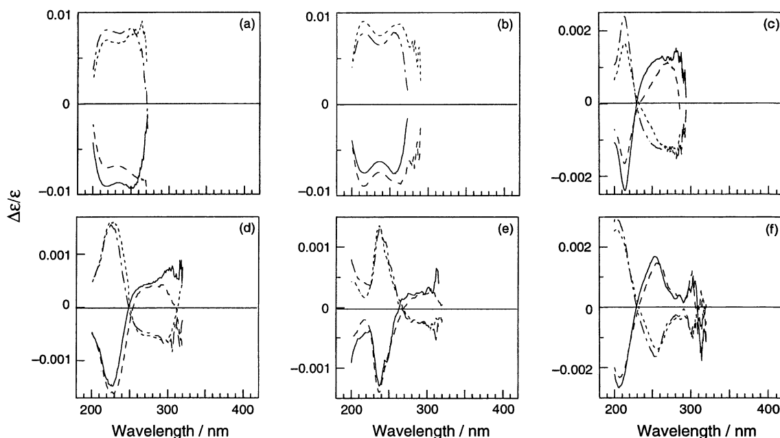
Fig. 7. Anisotropy ( g ) factors of (–)– and (+)–quadracyclanes in hexane (solid and chain, respectively) and in acetonitrile (dash and short dash, respectively): (a) 1b , (b) 2b , (c) 3b , (d) 4b , (e) 5b , and (f) 6b .
